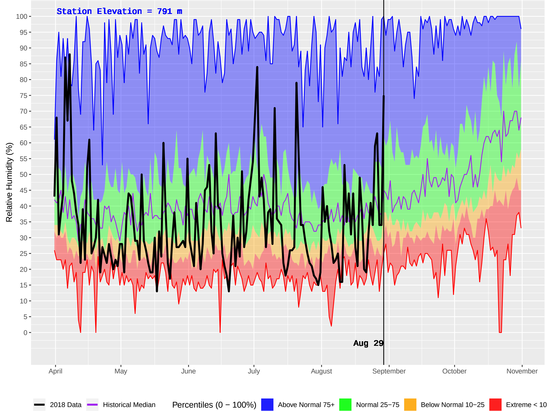
ALEXIS CREEK (209) : Historical (1980–2016) and Current (2018) Daily Relative Humidity
