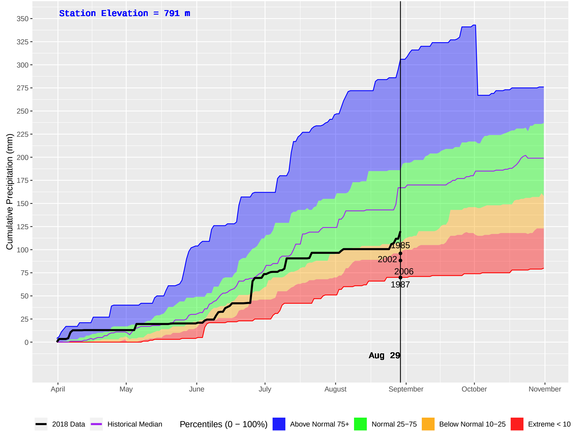
ALEXIS CREEK (209) : Historical (1980–2016) and Current (2018) Daily Cumulative Precipitation
