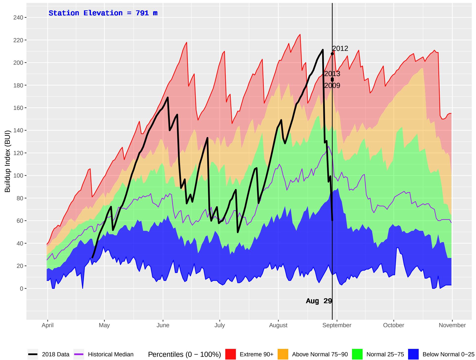
ALEXIS CREEK (209) : Historical (1980–2016) and Current (2018) Daily Buildup Index (BUI)
