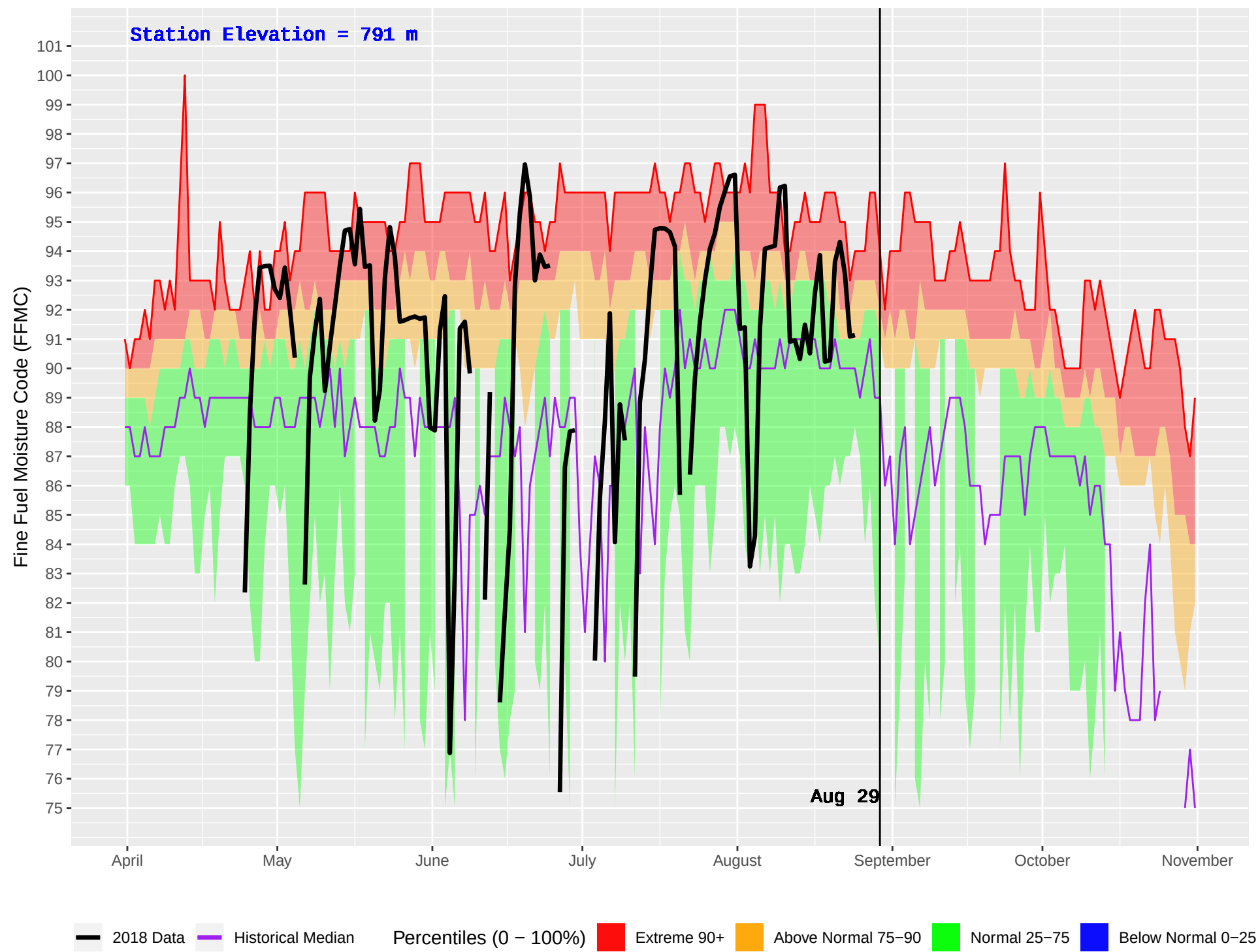
ALEXIS CREEK (209) : Historical (1980–2016) and Current (2018) Daily Fine Fuel Moisture Code (FFMC)
